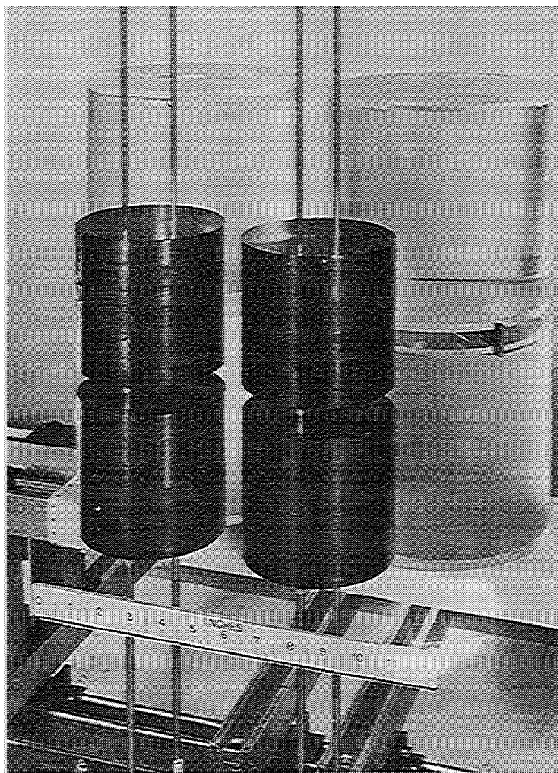
FIG. 6. Composite array of four 20.9 kg U(93.2) metal units and four 2.1 kg U(92.6) units of \text{UO}_2(\text{NO}_3)_2 solution.
