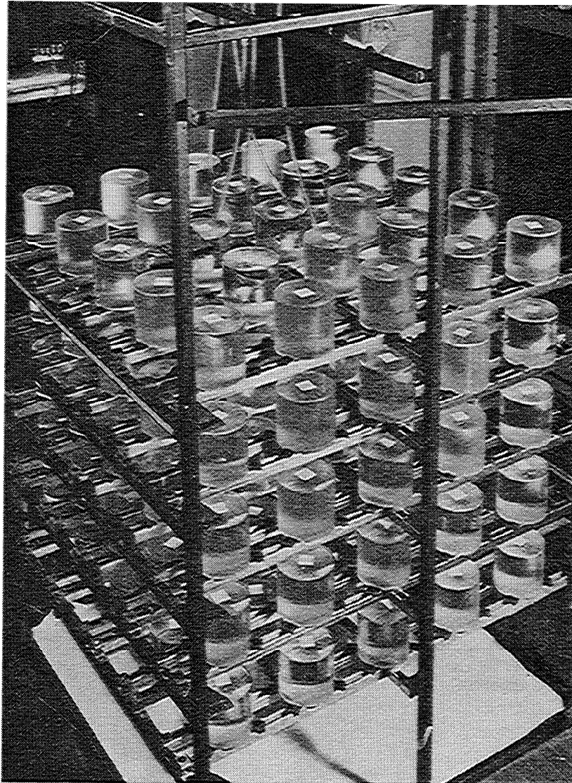
FIG. 1. A view of a critical system of 125 F^1 -units of Series III experiments. Each unit contains 1.92 kg of ^{235}\text{U} as uranyl nitrate solution.
