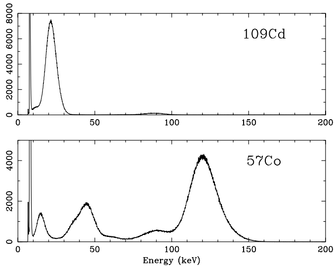
Fig. 10. Pulse-height spectra of ^{109}\text{Cd} (top) and ^{57}\text{Co} (bottom) for BGO readout with APD.
