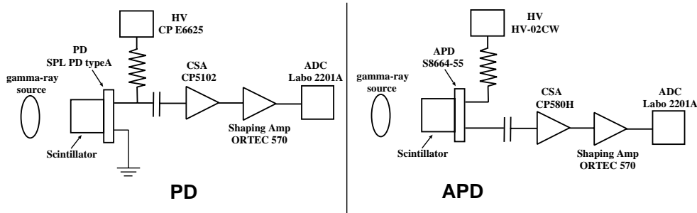
Fig. 2. Setup Diagrams of measurements for PD (left) and APD (right).
