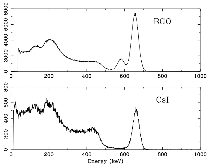
Fig. 8. Pulse-height spectra of ^{137}\text{Cs} for scintillators readout with APD; BGO (top) and CsI (bottom).
