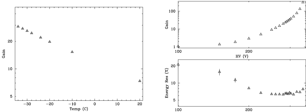
Fig. 12. The left is the temperature dependence of APD gain at -30^{circ}C , and the right is the bias dependence of APD gain (top) and energy resolution (bottom) for the 662 keV gamma-ray.
