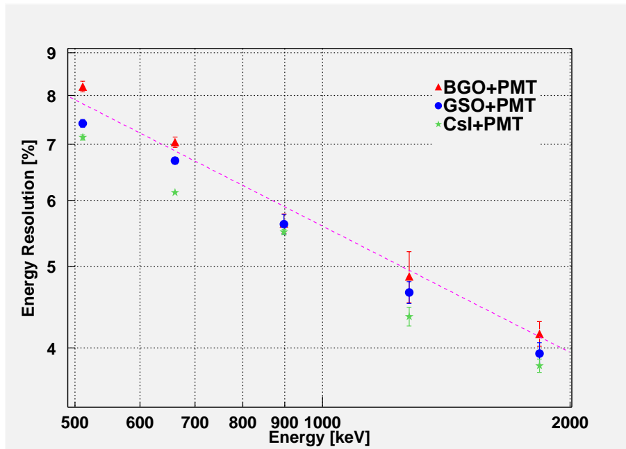
Fig. 4. Energy resolution (FWHM) of scintillators readout with PMT against the gamma-ray energy. The dashed line represents the relation of \propto E^{-0.5} .
