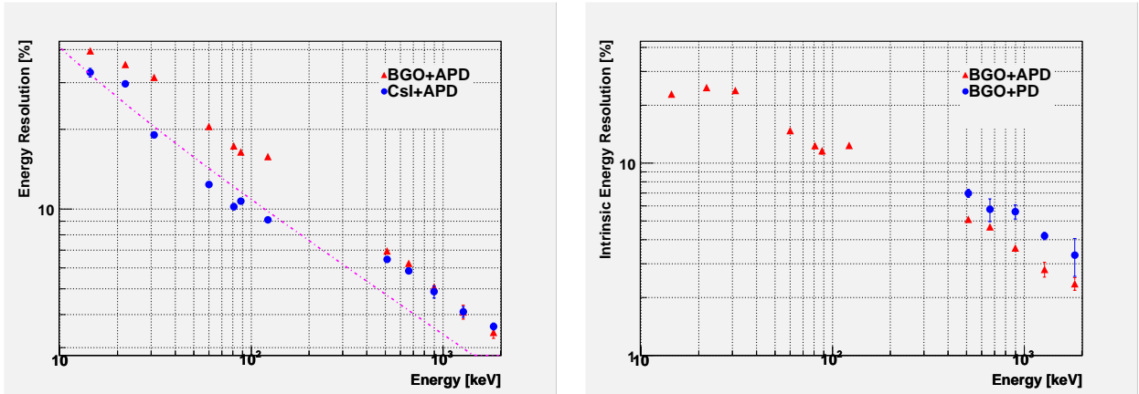
Fig. 11. (Left) Energy resolution (FWHM) of CsI and BGO readout with APD against the gamma-ray energy. The dashed line represents the predicted relation for BGO. (Right) The calculated \delta_{sc} as a function of the gamma-ray energy for BGO readout with APD.
