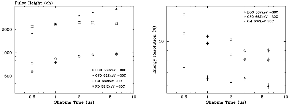
Fig. 5. Pulse-height (left) and Energy resolution (right) of ^{137}\text{Cs} against the shaping time \tau . for scintillators readout with PD.
