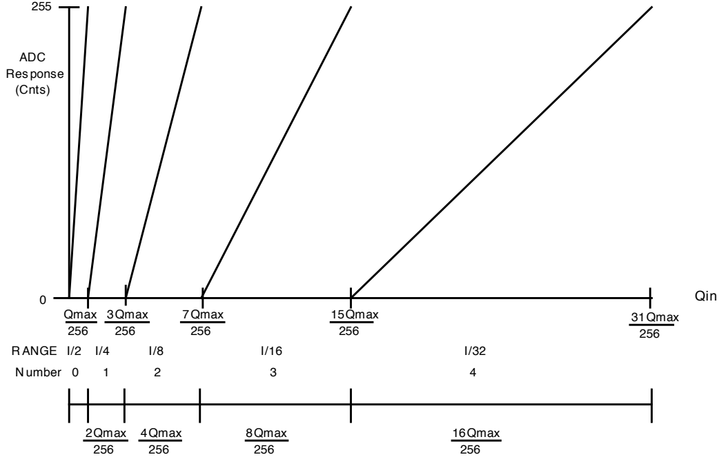
Fig. 28. Response of the QIE-chip based electronics: The x-axis shows the amount of charge injected into the chip, while the y-axis shows the ADC response for the different ranges. Only the first five out of the eight ranges are shown.
