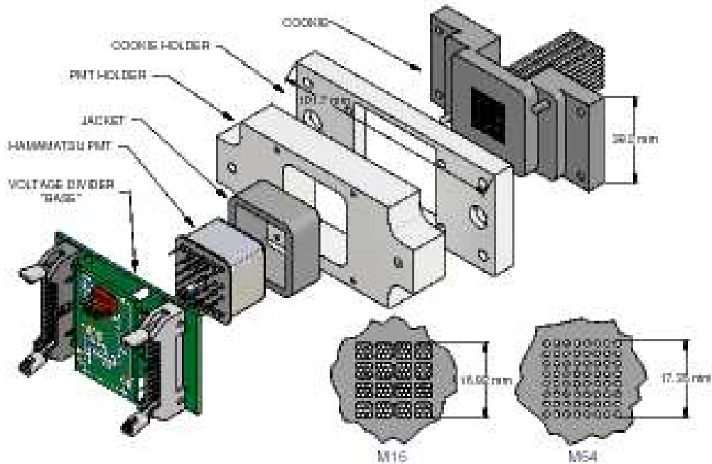
Fig. 18. The M16 PMT mounting assembly, one of three inside each far detector MUX box. The near detector M64 mounting assembly is identical except that only one fiber is placed on each pixel. The fiber “cookie” layouts used in the two cases are shown face-on in the lower right of the figure.
