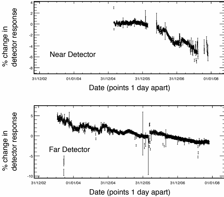
Fig. 34. Drifts in the responses of the near (top) and far (bottom) detectors. Each point is the percentage drift of one day's data from an arbitrary zero point of the daily median pulse height per plane of through-going cosmic ray muons. The errors bars show the rms spreads of the daily pulse heights per plane. The gap in the data corresponds to the summer 2006 shutdown.
