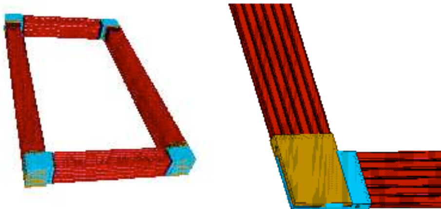
Fig. 6. Sketches of the four legs of the near detector coil assembly (left) and of one lap joint between two coil planks (right).
