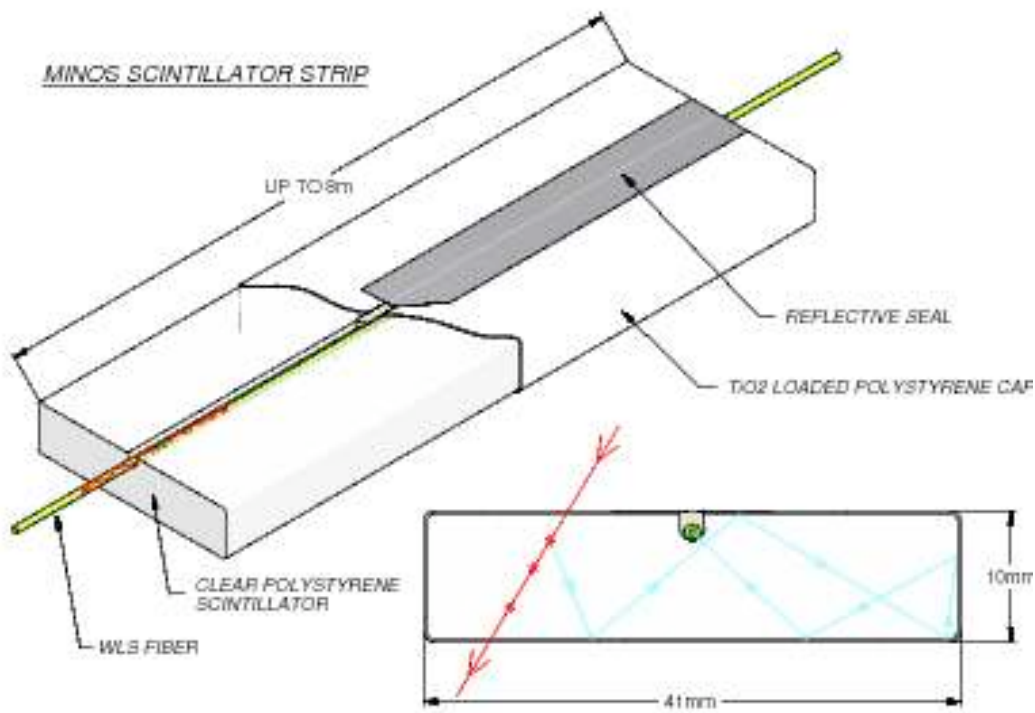
Fig. 9. Cutaway drawing of a single scintillator strip. Light produced by an ionizing particle is multiply reflected inside the strip by the 0.25 mm-thick outer reflective coating (shown in the cross-section view). Light absorbed by a WLS fiber is re-emitted isotropically. Those resulting waveshifted photons whose directions fall within the total internal reflection cones are transported along the fiber to the edges of the detector, subsequently being routed to the photodetectors (Fig. 8).
