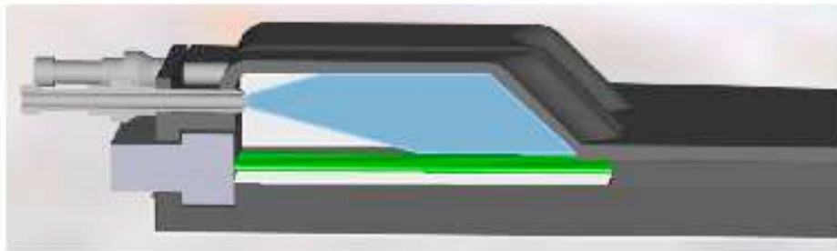
Fig. 31. A cutaway view of the light-injection module. A curtain of up to ten green WLS fibers runs across the bottom of the LIM cavity, and the injected light illuminates them from above. The T-shaped component at the lower left is the bulk optical connector into which the WLS fibers are glued. In the upper left foreground is a cutaway of one of the connectors terminating the light-injection fibers; another connector is visible behind it.
